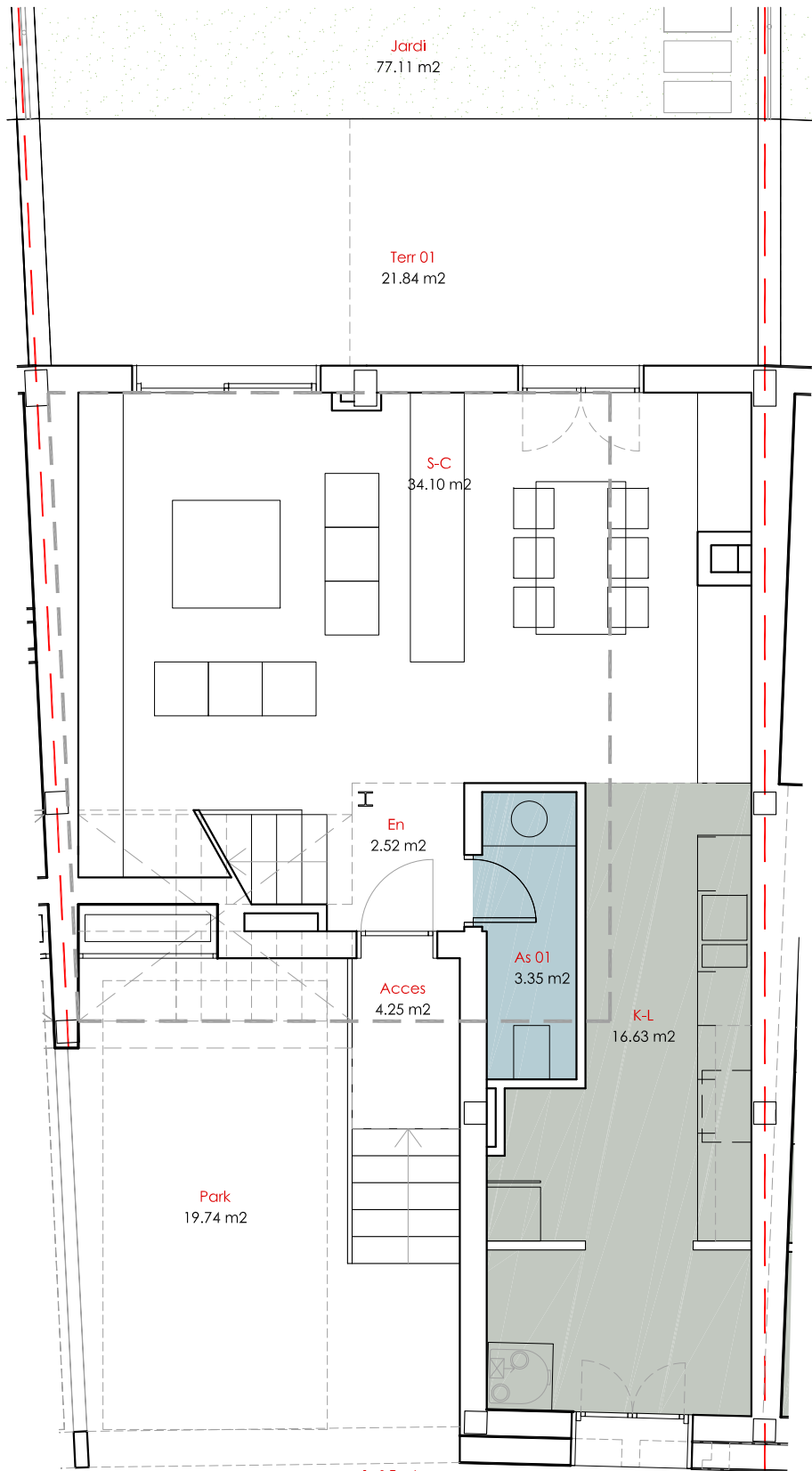
Ground floor
